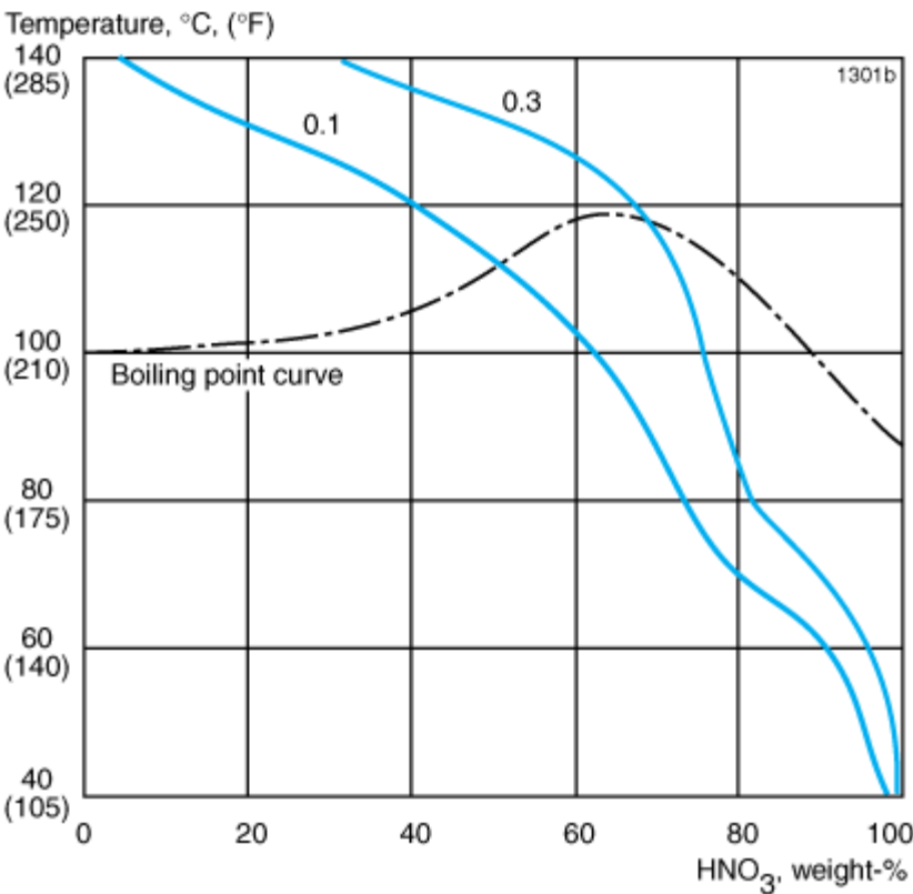
Figure 2. Diagram showing isocorrosion in nitric acid for Alleima
