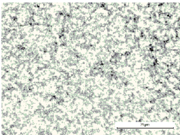
Figure 2. Alleima® 13C26 hardened and tempered.
