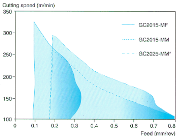
Figure 1. Machining chart for Sanmac 4435.
