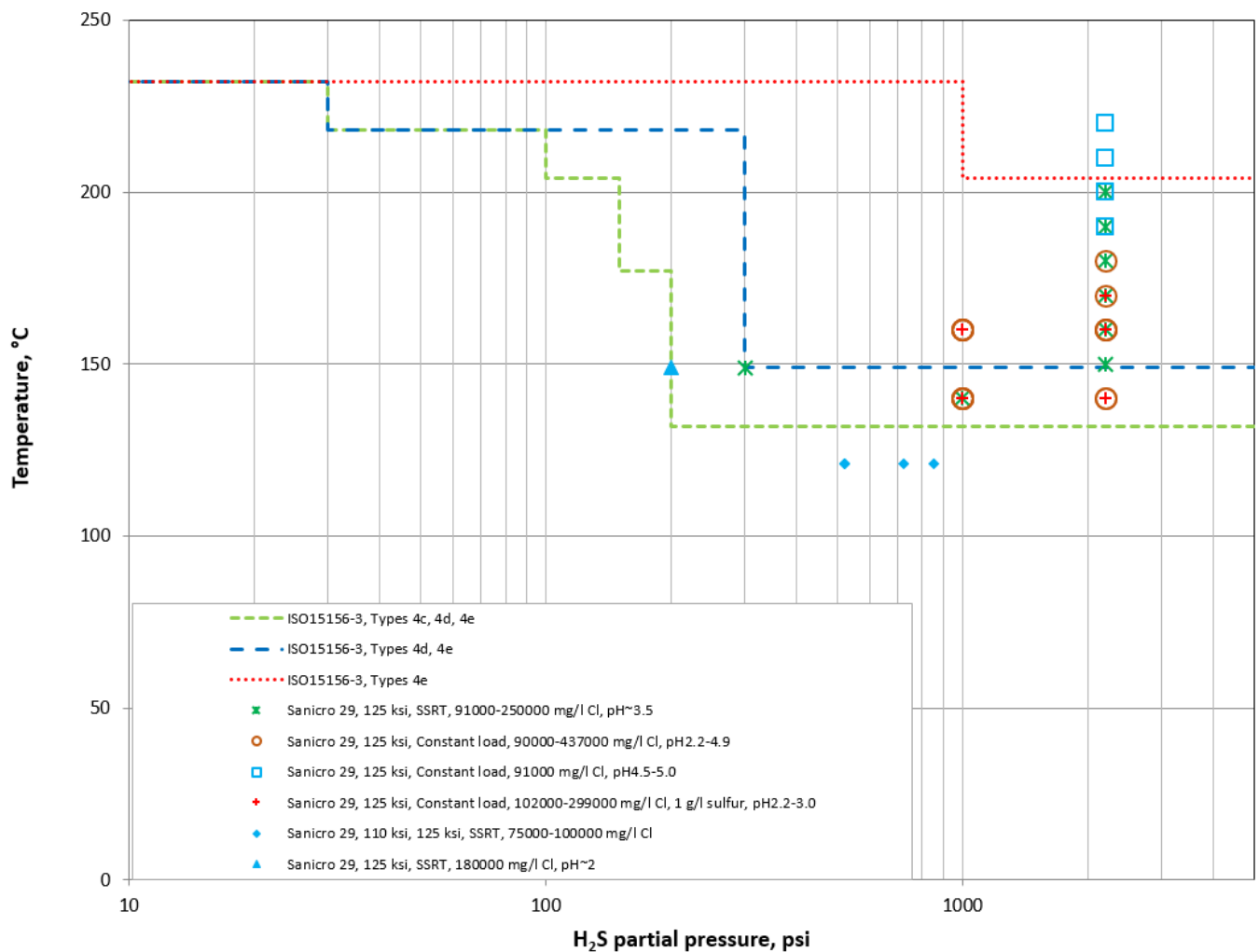
Figure 3: SCC testing data of cold worked Sanicro® 29 tube materials in sour environments in comparison with the ISO 15156-3 limits for 4c type materials. The SCC testing has been performed on Sanicro® 29 tube materials stressed at 100% actual yield strength (AYS) using tensile constant load per NACE TM0177 method A, as well as slow strain rate test (SSRT) per NACE TM0198 at strain rate of 4 \times 10^{-6} in/in/sec. Sanicro® 29 showed good ductility in the tested sour environments with no failures.
