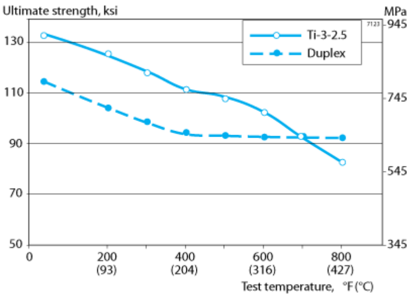
Figure 5 Temperature vs ultimate tensile strength for Ti-3-2.5 and duplex stainless steel tubing.
