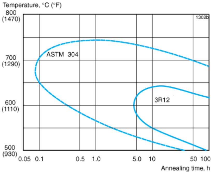
Figure 3. TTC-diagram for Alleima 3R12 (AISI 304L) and AISI 304.
