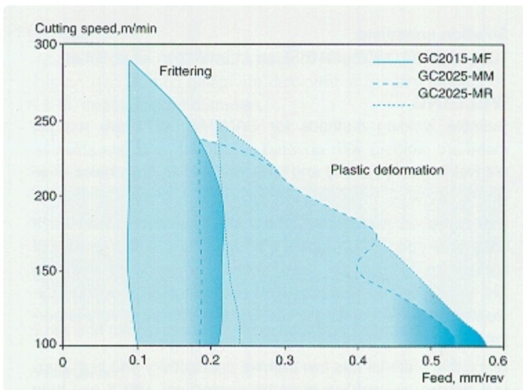
Figure 1. Machining chart for Sanmac 4571.
